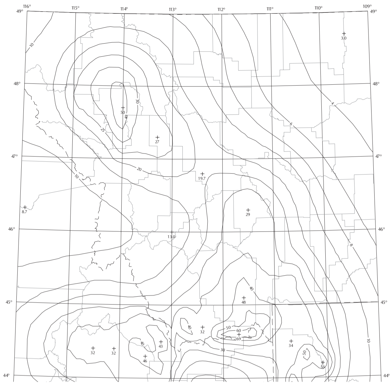
FIGURE 1615 (6) MAXIMUM CONSIDERED EARTHQUAKE GROUND MOTION FOR REGION 2 OF 1.0 SEC SPECTRAL RESPONSE ACCELERATION (5% OF CRITICAL DAMPING), SITE CLASS B
